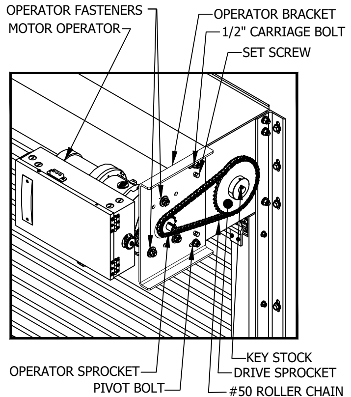
FIGURE C-2 McKEON OPERATOR
