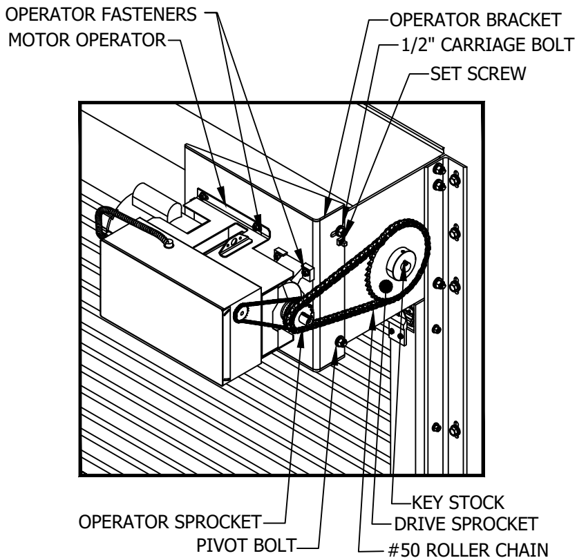
FIGURE C-1 LIFTMASTER OPERATOR
